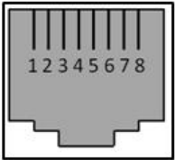
RJ45 Port
